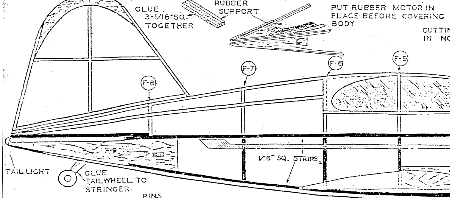
SIDE VIEW
