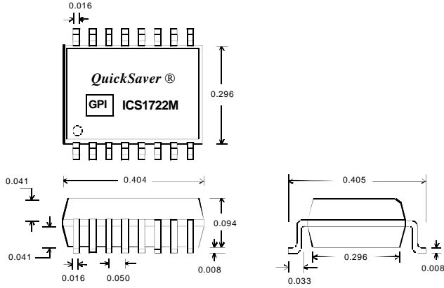
All package dimensions are in inches. 16-Pin SOIC Package (300 mil)
